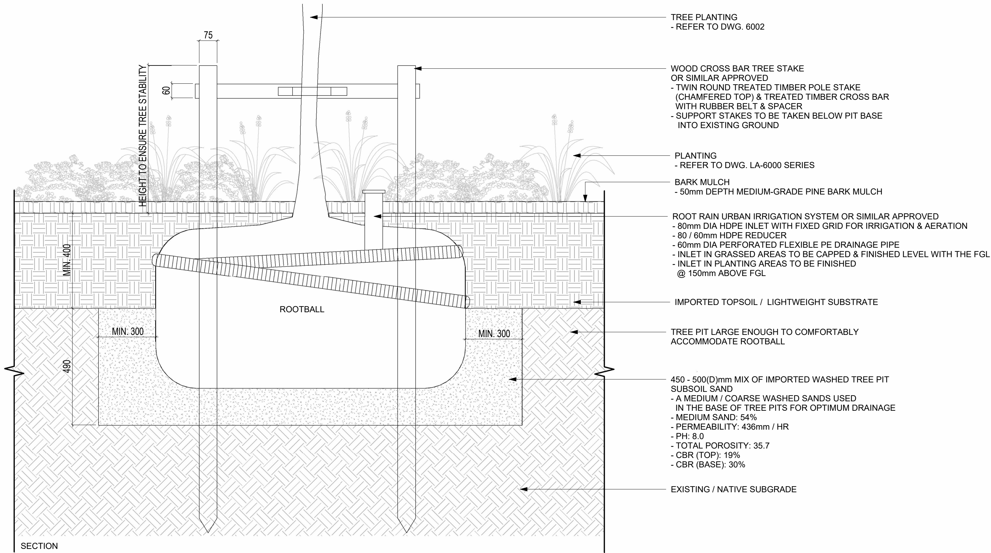
1 TYPICAL DETAIL: TREE PIT IN NATURAL GROUND WITH TREE STAKING SYSTEM1 SCALE: 1:10 @A1
